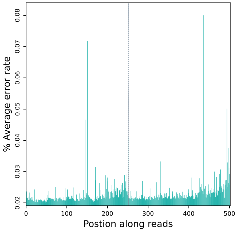
Error rate distribution along reads (R10103)
